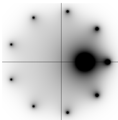
Figure 1: Plot of the Generating function for the set of bitstrings having no occurrence of the pattern 000000001
