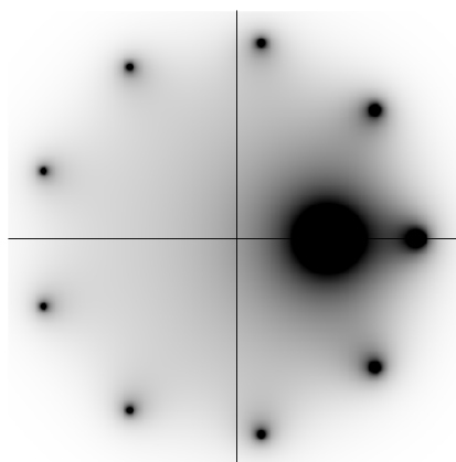
Figure 2: Plot of the Generating function for the set of bitstrings having no occurrence of the pattern 01010101
