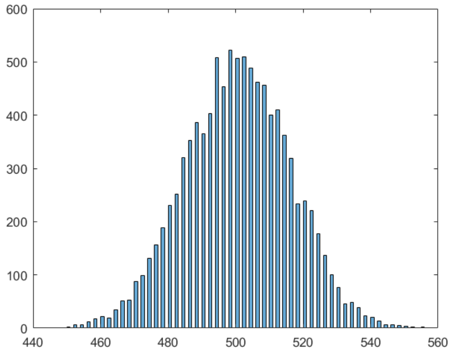
Figure 3: t = 10^5
