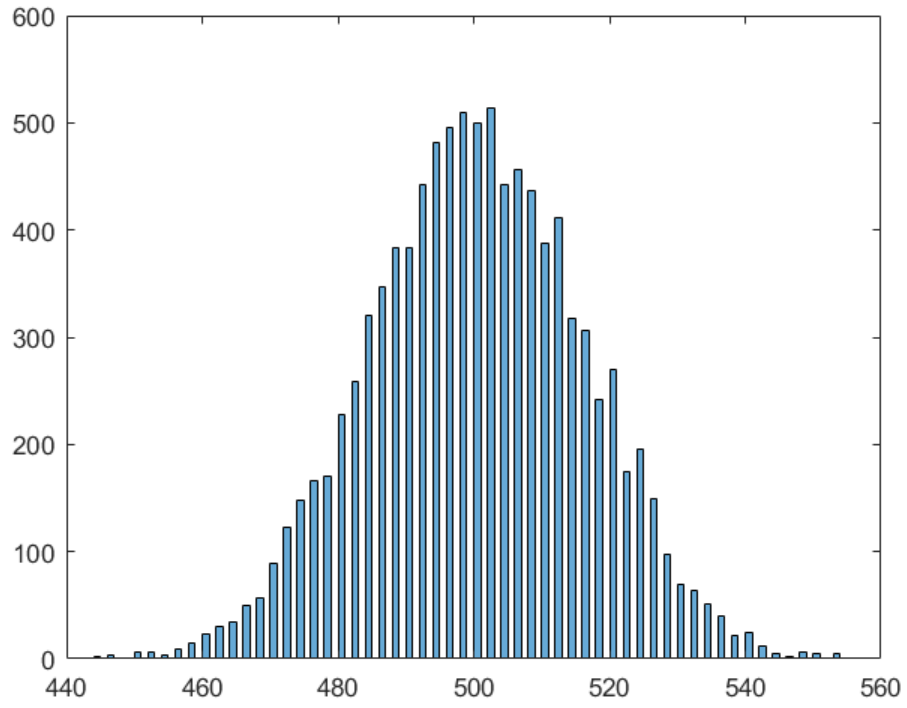
Figure 2: t = 10^4
