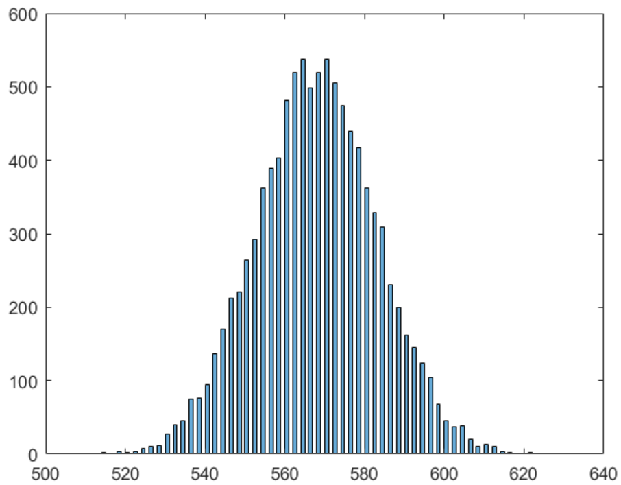
Figure 1: t = 10^3
